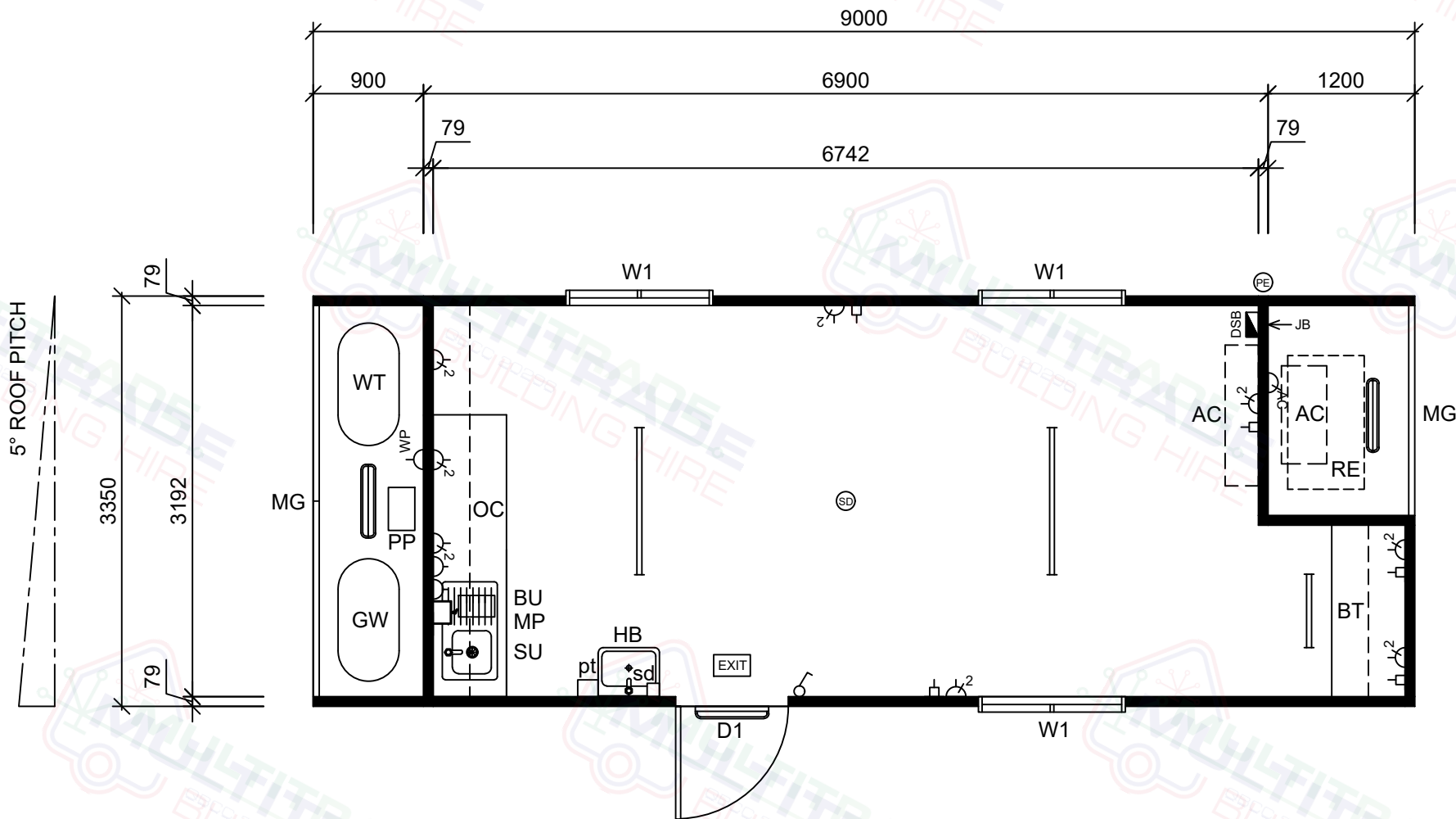
9.0x3.35m Solar Facility - Floor Plan
